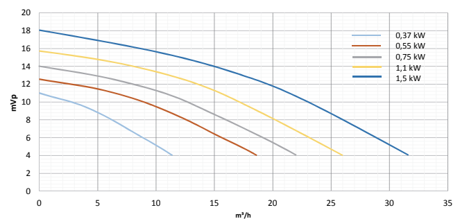
Pump capacities
