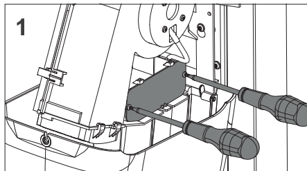
Detach the circuit print control cover
