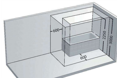
Electrical protected areas in the bathroom
